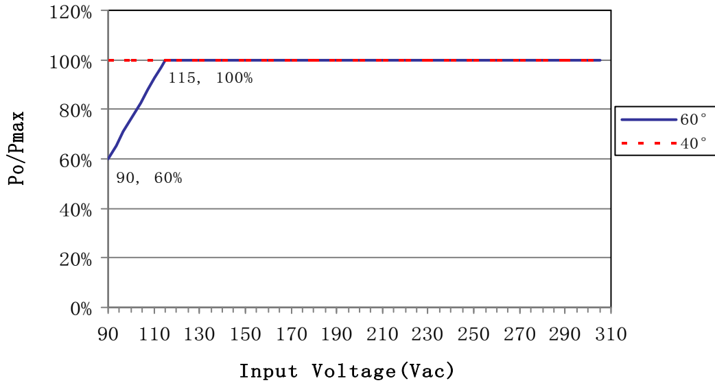
Po/Pmax VS Input Voltage Curve
