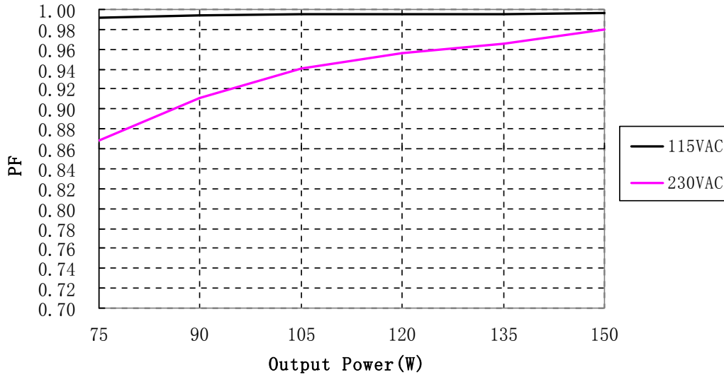
Power Factor VS Output Power Curve
