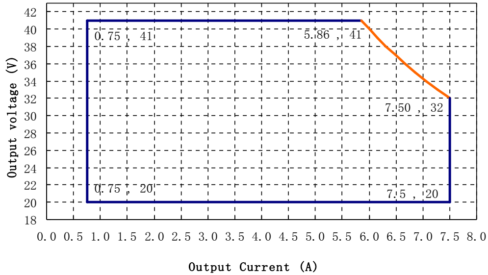
Output Voltage VS Output Current Curve
