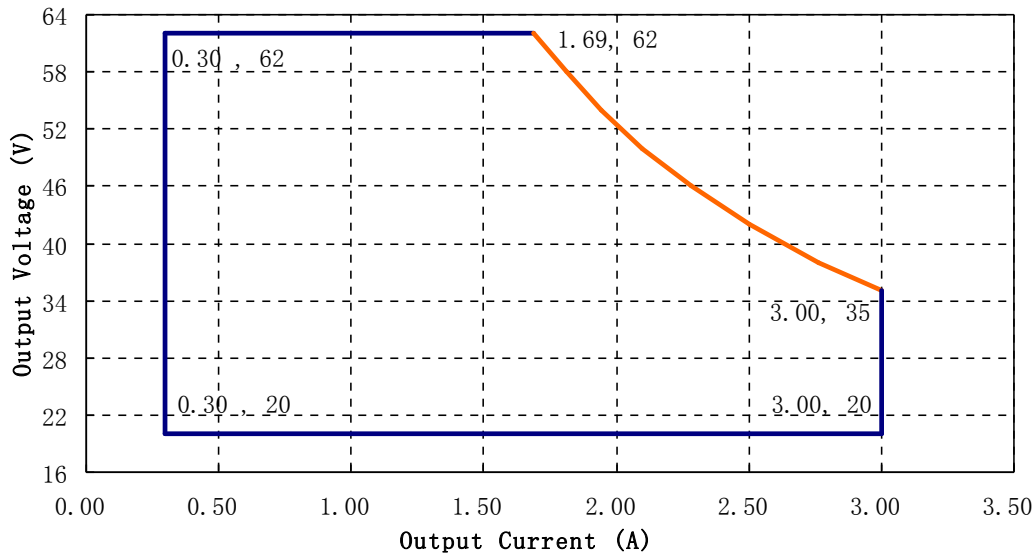
Output Voltage VS Current Curve
